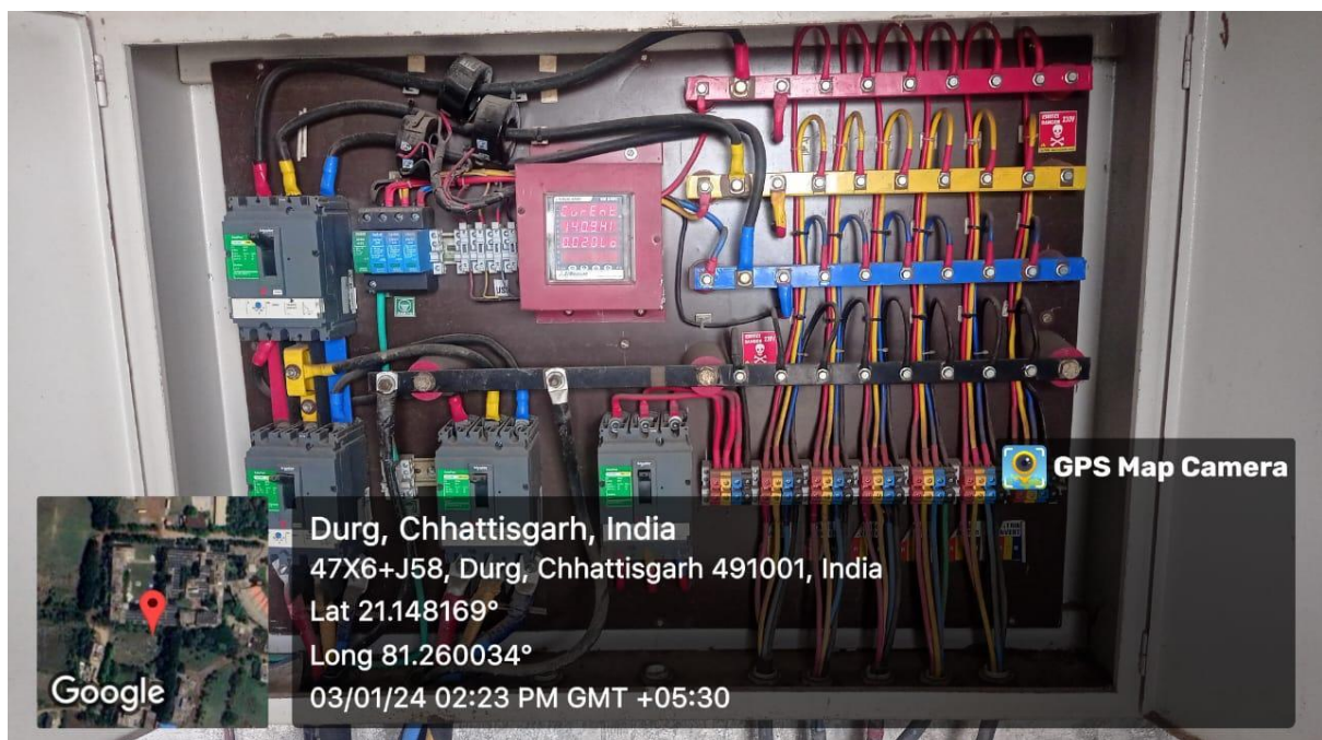
Main Circuit Panel of Solar with readings
